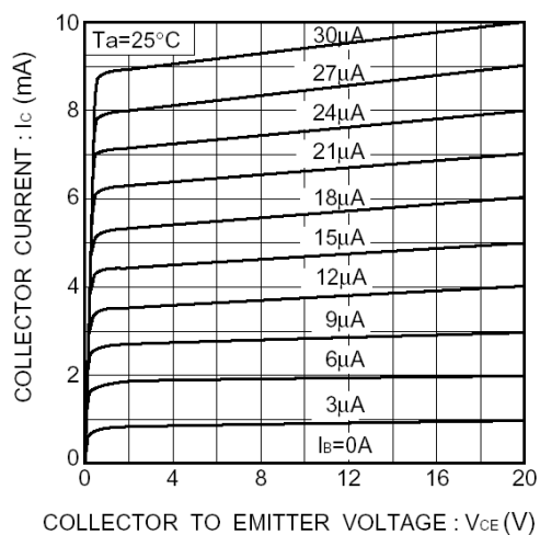
Fig.3 Grounded emitter output characteristics ( II )
