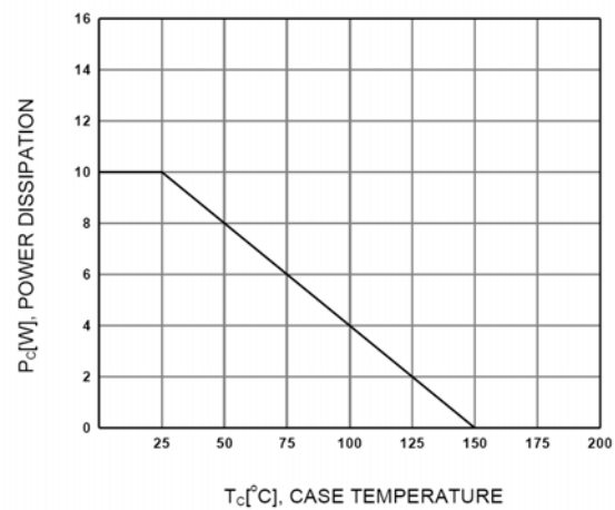
Figure 8. Power Derating
