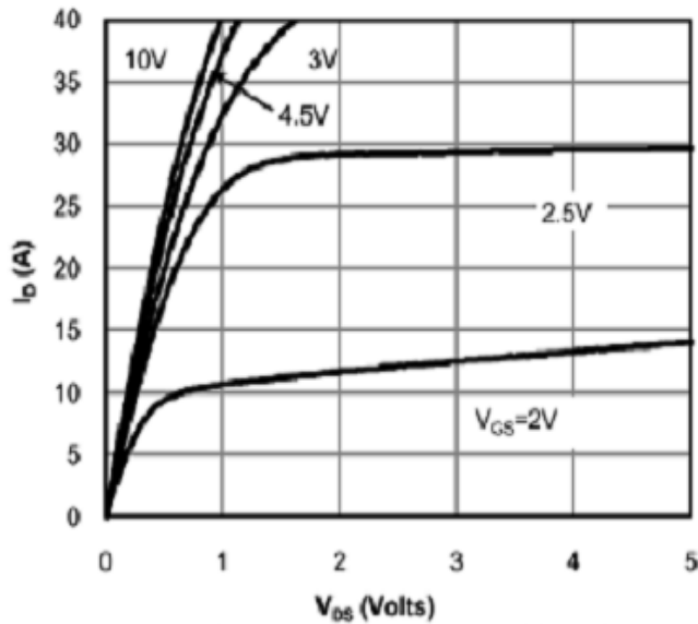
Fig 1: On-Region Characteristics (Note E)
