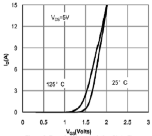
Figure 2: Transfer Characteristics (Note E)
